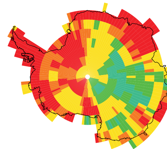
RMS % change in ICE relative to BASE (bsnow)
