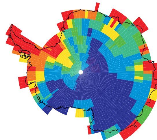
RMS % change in MET relative to BASE (bsnow)
