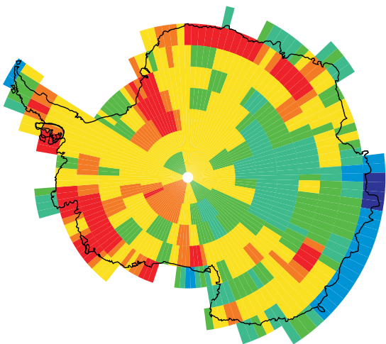
RMS % change in ICE relative to BASE (total)
