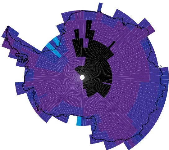
RMS % change in MET relative to BASE (total)
