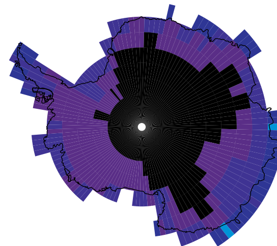
RMS % change in MET relative to BASE (ocean)
