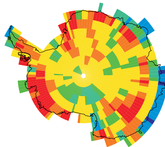
RMS % change in ICE relative to BASE (ocean)
