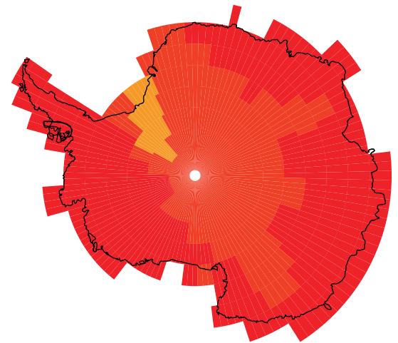
Mean % change in LGM2 relative to MET (bsnow)
