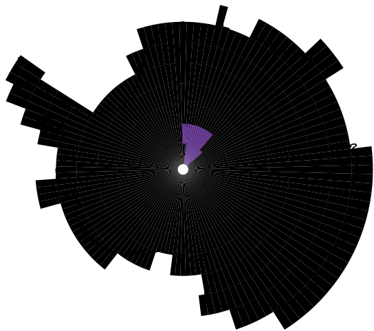
Mean % change in LGM1 relative to MET (total)
