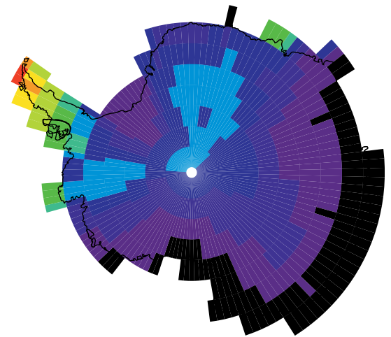
Mean % change in LGM1 relative to MET (bsnow)
