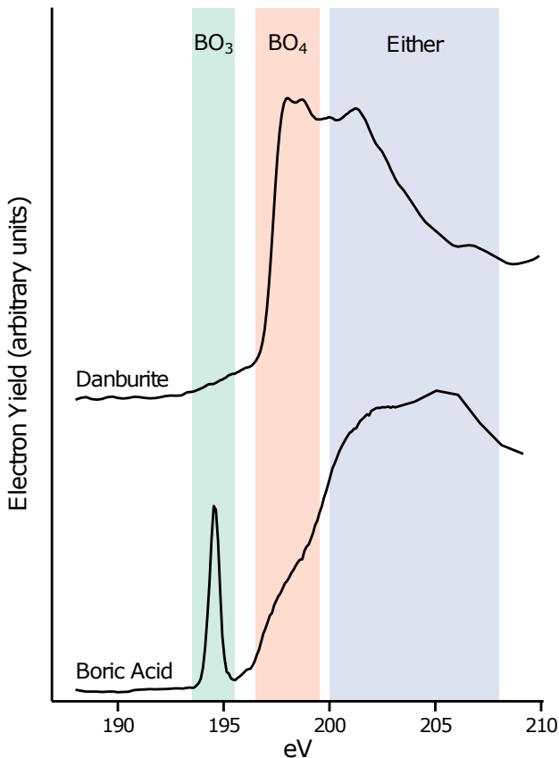
Figure S3: Spectra from danburite [ \text{CaB}_2(\text{SiO}_4)_2 ] and boric acid [ \text{B}(\text{OH})_3 ] reference materials show the positions of the trigonal and tetrahedral B peaks.
