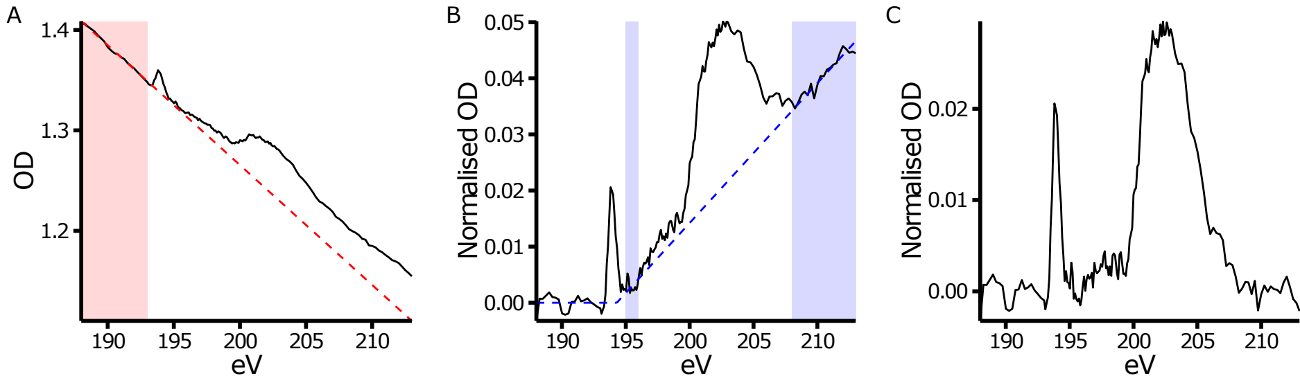
Figure S4: The two-step normalisation procedure described by Fleet et al. (2000), as applied to our data. (A) the un-normalised spectrum with the first correction line fitted to the pre-edge region shown in red. (B) The intermediate spectrum after subtraction of the red line in A with a second normalisation line based on the shaded blue regions shown. (C) The final, normalised spectrum.
