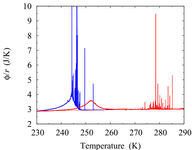
FIG. 2. DTA traces for heating (red) and cooling (blue) experiments. Data corresponding to cooling experiments have been changed in sign to allow a better comparison to heating data.
